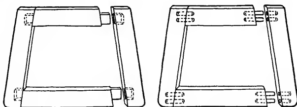
FIG. 398. CHAIR SEAT FRAME.
